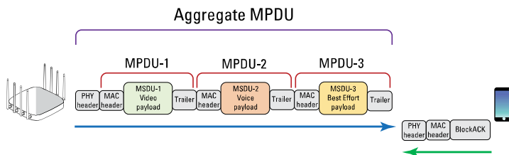
FIGURE 5-5: Multi-TID AMPDU.
