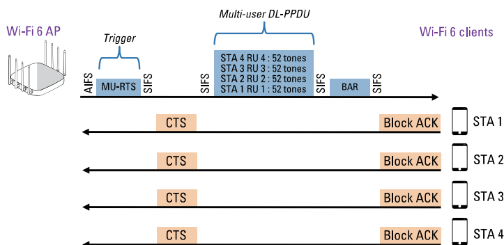
FIGURE 2-9: Downlink OFDMA.
