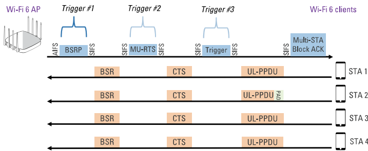
FIGURE 2-10: Uplink OFDMA.
